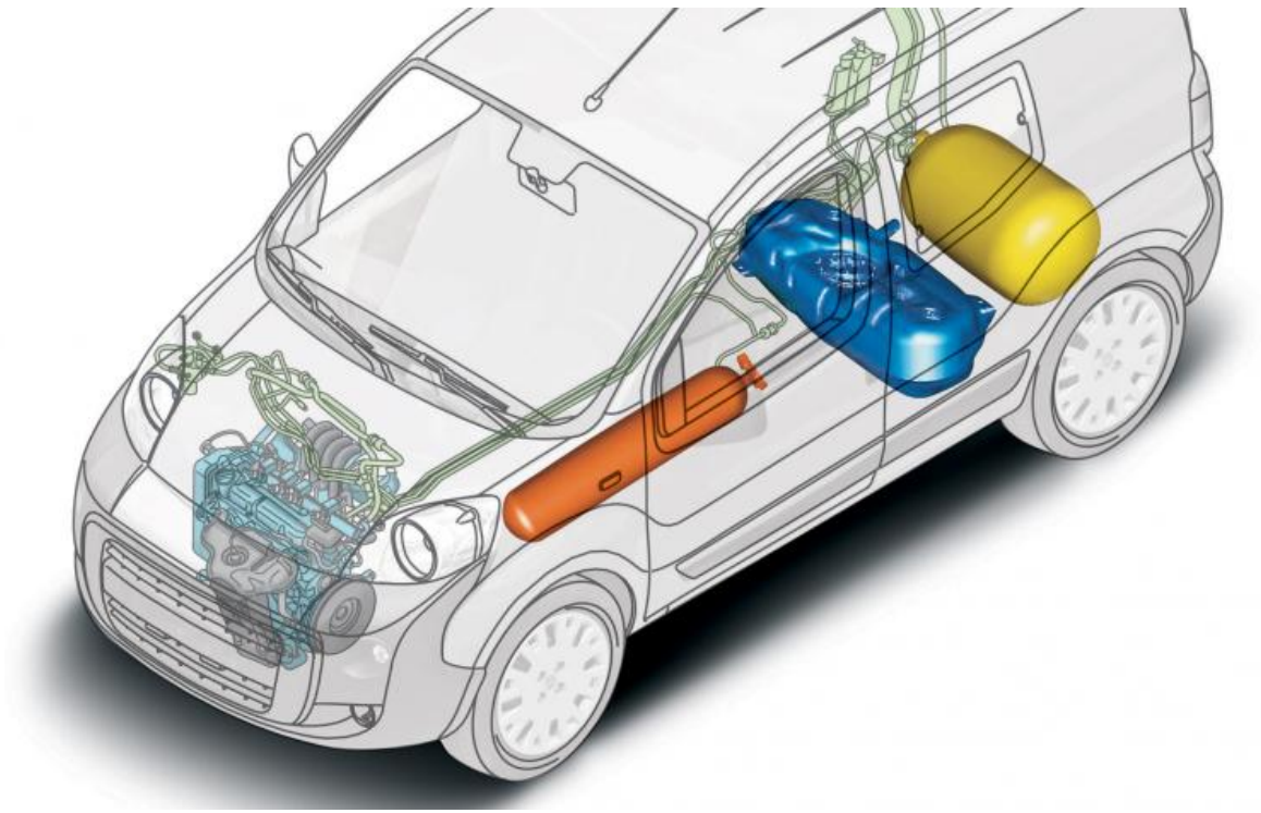
Fiat Professional Fiorino Natural-Power
